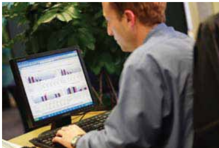
Management Interface
